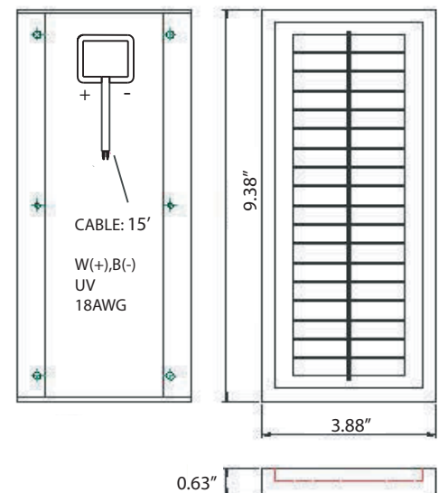
Power Up 1 Watt Module
